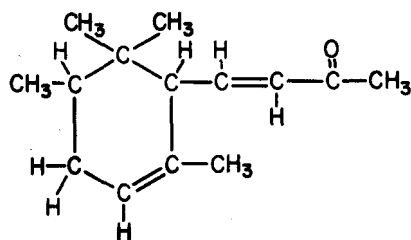
Fig. 1-10. The substance pictured is α-ionone.
