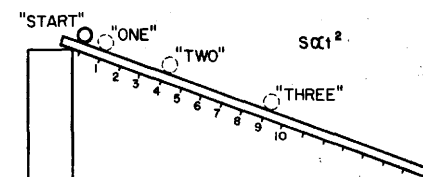
Fig. 5-1. A ball rolls down an inclined track.
